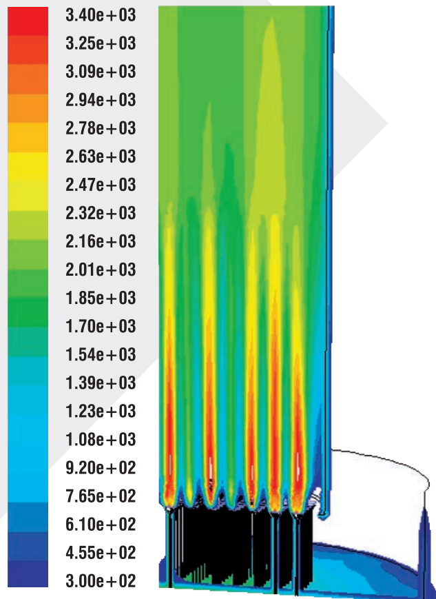
CFD No Wind Results – Centerline Temperature (°F)
