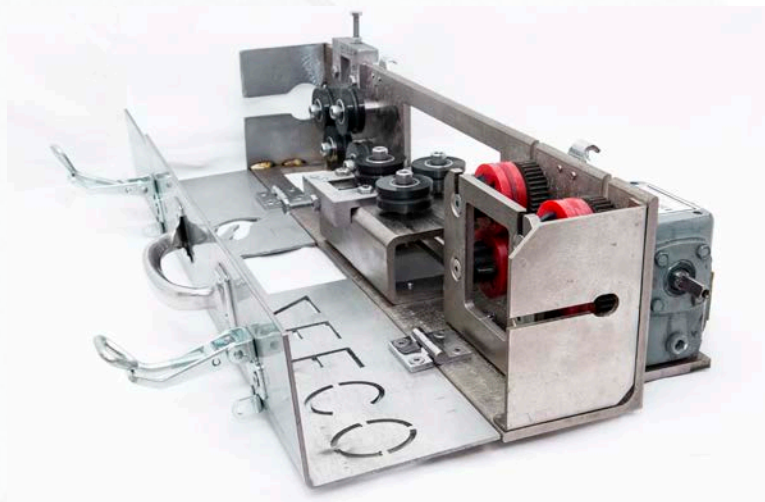
The ZEECO Navigator Thermocouple Pusher/Straightener Device
